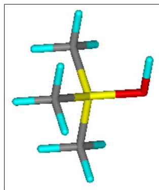
reaktant
