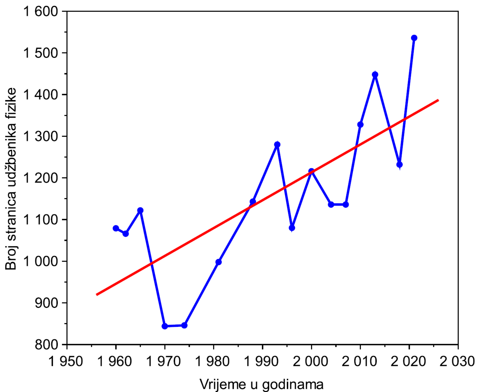
Udžbenik „raste”: Fundamentals of Physics (D. Halliday, R. Resnick) Pravac: Y = 6.688(1651)X - 12164(3289) , F = 16 , R = 0.7345 , p < 0.003
