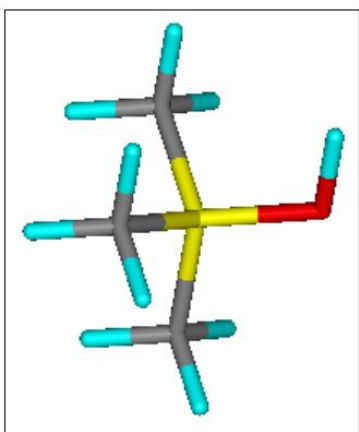
reaktant
